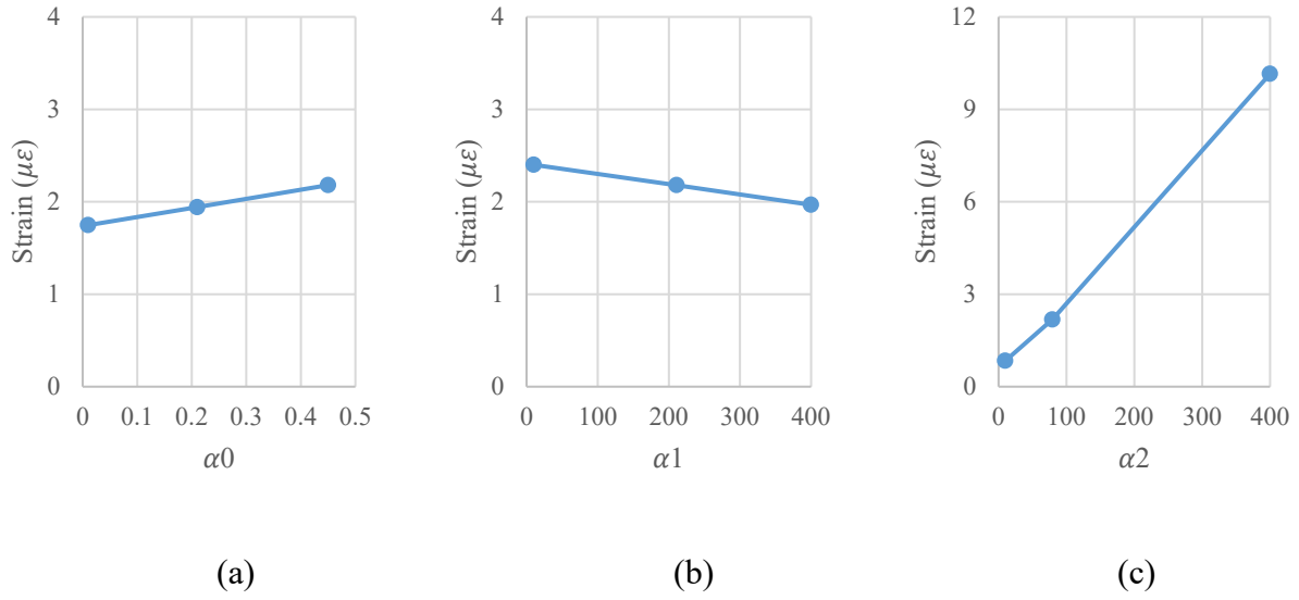
Figure 1.11 Effect of thermal expansion coefficients (unit: \times 10^{-6} ) of (a) fiber core (b) inner coating (c) outer coating on the fiber core strain
