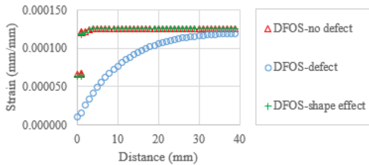
Figure 3.20 Strain distribution of the optical fiber along the center path
