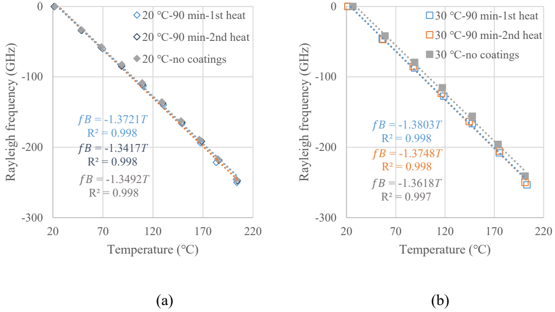
Figure 1.9 Rayleigh frequency-temperature curves before 200 °C with temperature increment of (a) 20 °C (b) 30 °C
