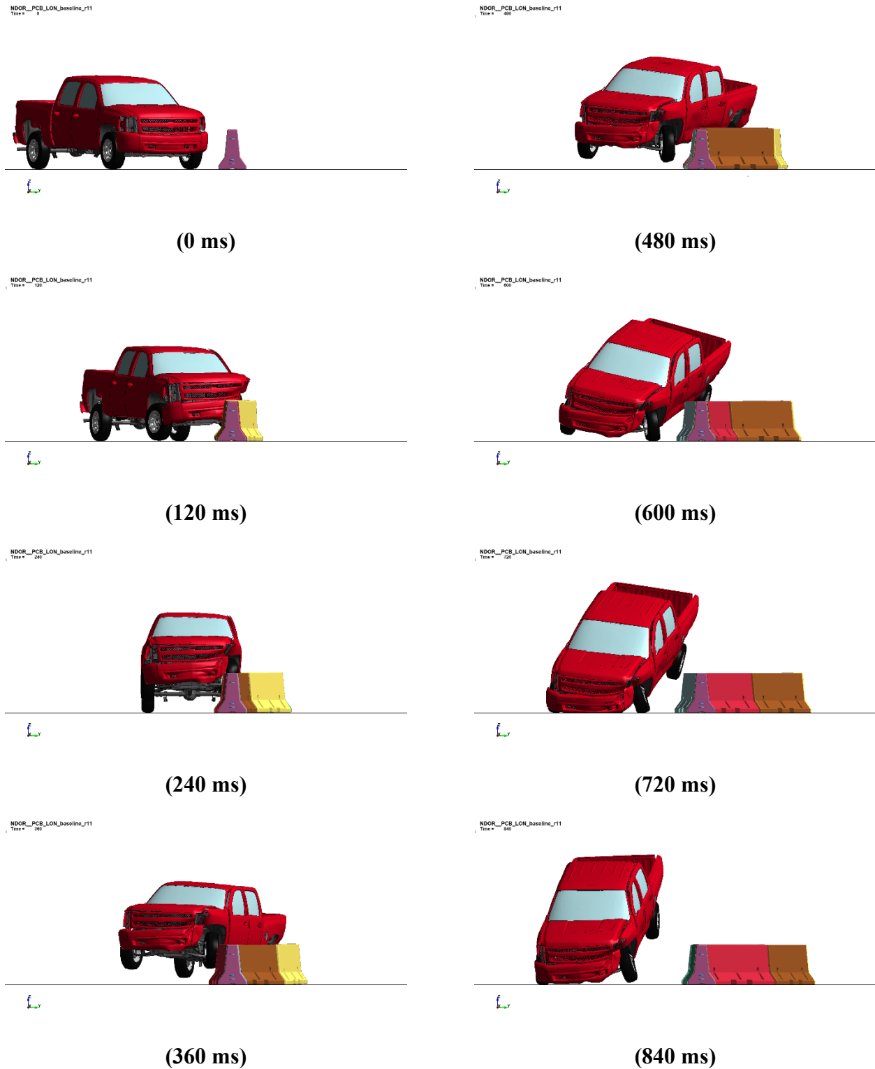
Figure 4.17 Sequential Images of Baseline F-Shape PCB Simulation
