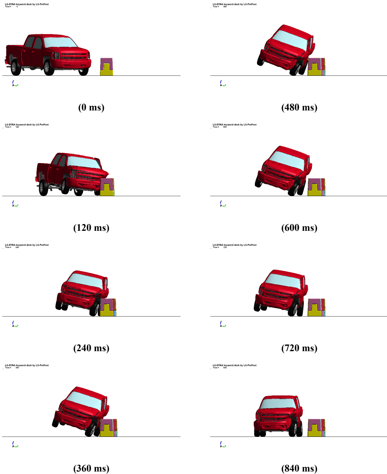
Figure 4.30 Sequential Images of Concept No. 19A Simulation
