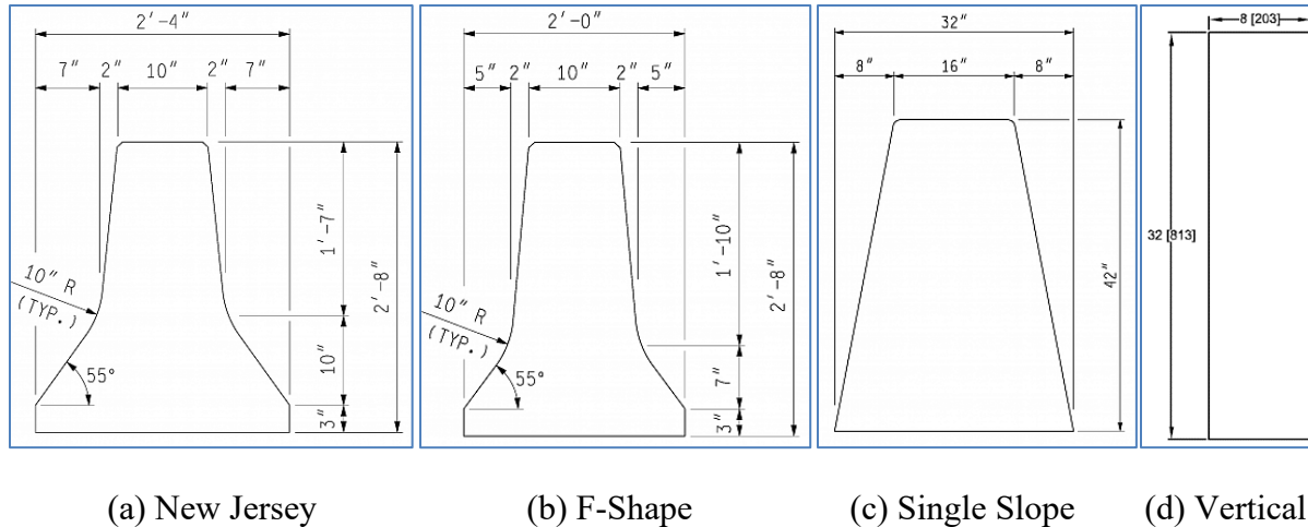
Figure 2.2 Typical PCB Shapes (a) New Jersey, (b) F-Shape, (c) Single Slope, and (d) Vertical
