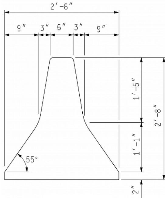
Figure 2.1 GM Shape PCB [9]
