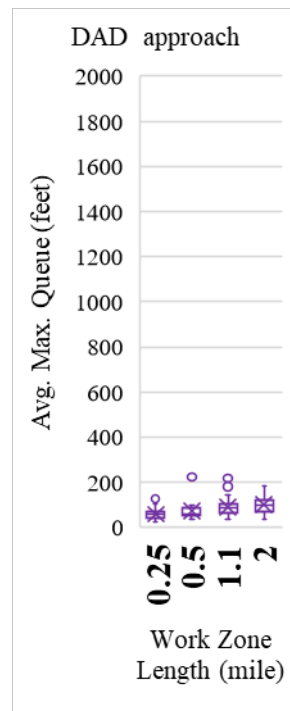
c. Queue for V_{Comb} of 150_25
