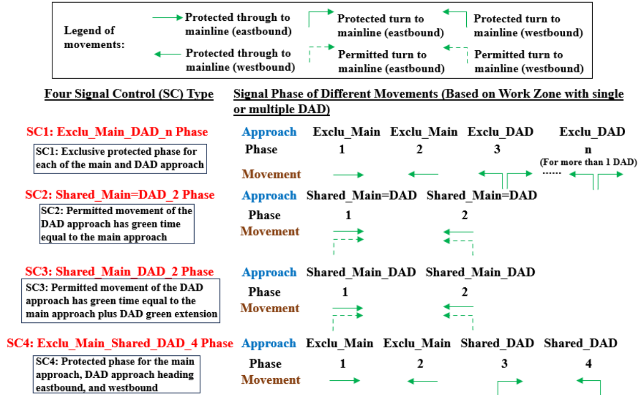
Figure 4.1 Phase and movement of four signal control strategies for DAD-operated work zone
