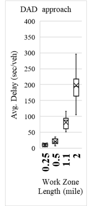
b. Delay for V_{Comb} of 50_100
