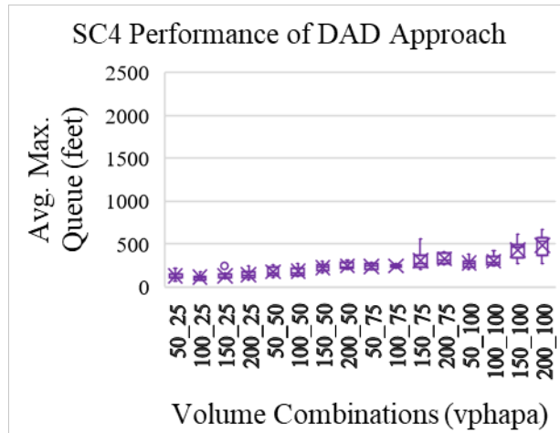
Figure A.8 Average maximum queue for All, Main and DAD approach under SC3 and SC4 for Main approach volume increase for various levels of constant DAD approach volume (WZL=1.1 mile, N_{DAD}=1 , T_{M\%}=20 , T_{DAD\%}=5 )
